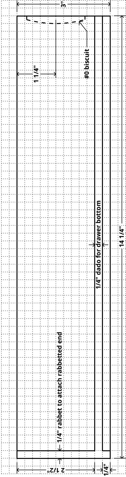
Toolbox side - lay out on 3 x 16 x 1/2" wood
